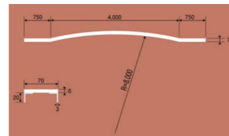
FA-7043 やり投げ用円弧
